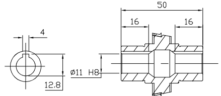
OUTPUT HOLLOW SHAFT
