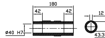
OUTPUT HOLLOW SHAFT
